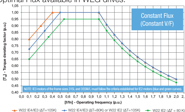
Figure 31 - Derating curves for constant flux condition
